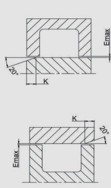
Closed groove-Piston seal
