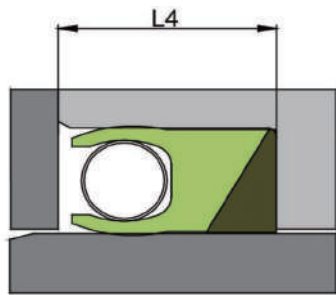
Triangular back-up ring
