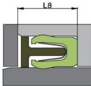
V shape supporting ring
