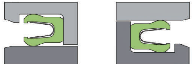
(Fig:4-2) Stepped groove
