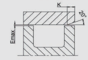
Closed groove-Piston seal
