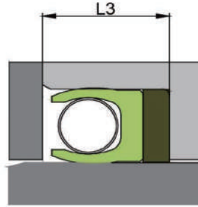
Rectangular back-up ring
