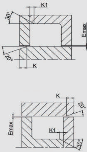
Open groove-piston seal
