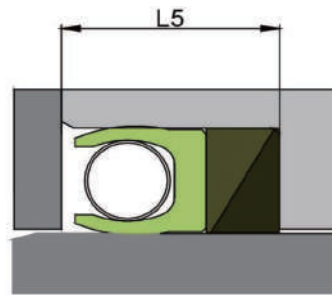
Double triangular back-up ring
