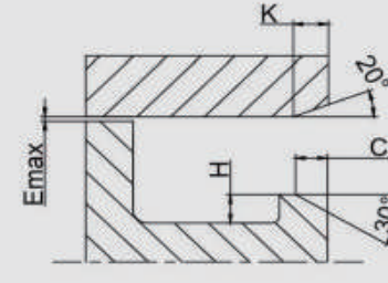
Stepped groove-Piston seal
