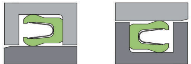
(Fig:4-3) Closed groove
