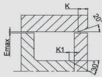
Open groove-piston seal
