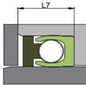
H shape supporting ring
