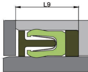
Back-up ring and supporting ring combination
